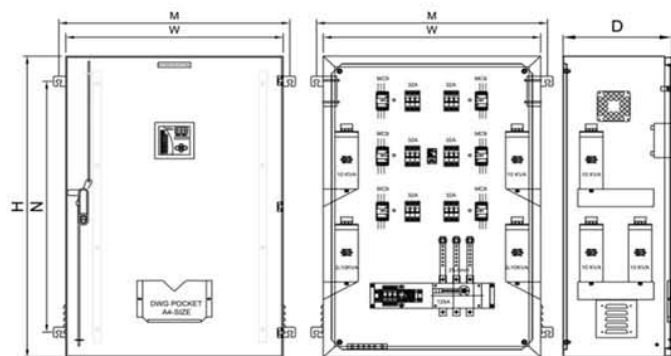
Capacitor Bank Panel 6 steps wall mounting
