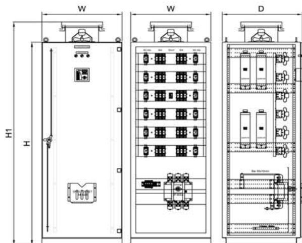
Capacitor Bank Panel 12 steps floor standing
